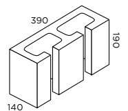
15.45 Clean Out 11.8kg 120 per pallet 1416kg pallet weight
