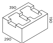
30.42 Trough Block 18.2kg 60 per pallet 1092kg pallet weight
