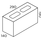
15.702 (reduced core) Three Quarter 12.9kg 128 per pallet 1651kg pallet weight
