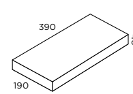
50.31 Capping Block 6.5kg 180 per pallet 1170kg pallet weight
