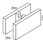
20.48 H Block 13.9kg 90 per pallet 1251kg pallet weight
