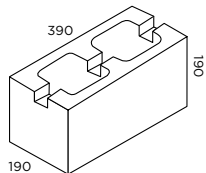
20.42 Trough Block 14.8kg 90 per pallet 1332kg pallet weight
