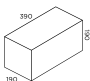
20.31 Full Length 30.1kg 54 per pallet 1626kg pallet weight
