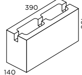
15.42 Trough Block 13.0kg 120 per pallet 1560kg pallet weight
