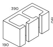
20.45 Clean Out 12.9kg 90 per pallet 1161kg pallet weight
