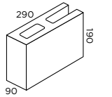
10.02 Three Quarter 7.7kg 240 per pallet 1848kg pallet weight
