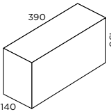
15.31 Full Length 21.6kg 72 per pallet 1555kg pallet weight
