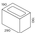
30.03/20.02 Half 12.6kg 120 per pallet 1512kg pallet weight
