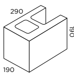
20.02/30.03 Three Quarter 12.5kg 120 per pallet 1500kg pallet weight
