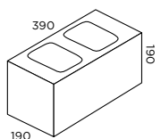
20.01 Full Length 16.2kg 90 per pallet 1458kg pallet weight
