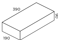
20.83/10.31 Full Length 14.2kg 108 per pallet 1534kg pallet weight
