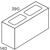
15.01 Full Length 12.5kg 120 per pallet 1500kg pallet weight
