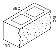
20.101 Full Length 17.0kg 90 per pallet 1530kg pallet weight
