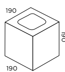
20.03 Half 7.9kg 180 per pallet 1422kg pallet weight
