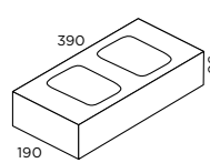
20.71 Full Length 7.3kg 180 per pallet 1314kg pallet weight
