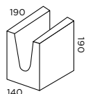
15.12 Lintel 7.0kg 240 per pallet 1680kg pallet weight
