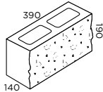
15.101 Full Length 15kg 120 per pallet 1800kg pallet weight
