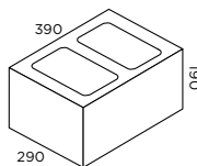
30.01 Full Length 19.5kg 60 per pallet 1170kg pallet weight
